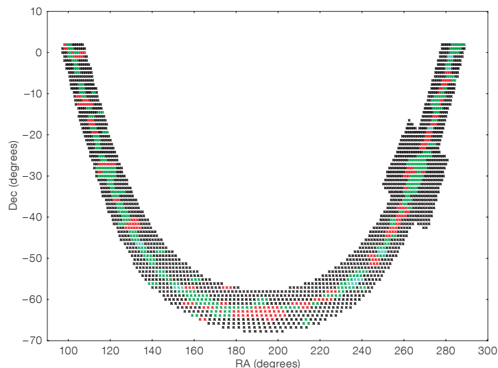
Figure 1. A map of the VPHAS+ survey footprint. The 2269 fields shown in black define the overall footprint, whilst those shown in green have already been completed. Red is used for fields observed only in H \alpha , r - and i -bands up to 30 September 2013, while blue is used for those observed only in u -, g - and r -bands.
